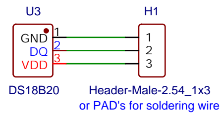
Optional temp sensor circuit
