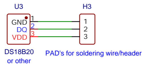
Optional temp sensor circuit
